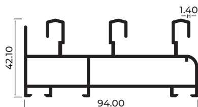
MARCO TRIPLE CORREDIZA VL4604
