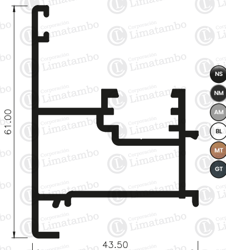
INVERSOR
