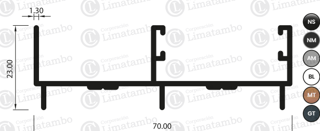
MARCO LATERAL
