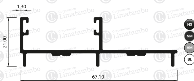
MARCO LATERAL
