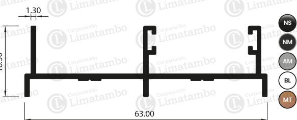
MARCO LATERAL
