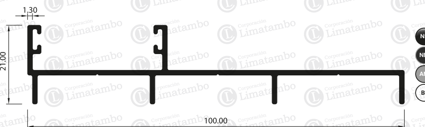
MARCO LATERAL TRIPLE CARRIL
