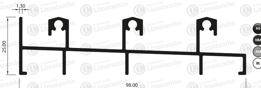
MARCO INFERIOR TRIPLE CARRIL
