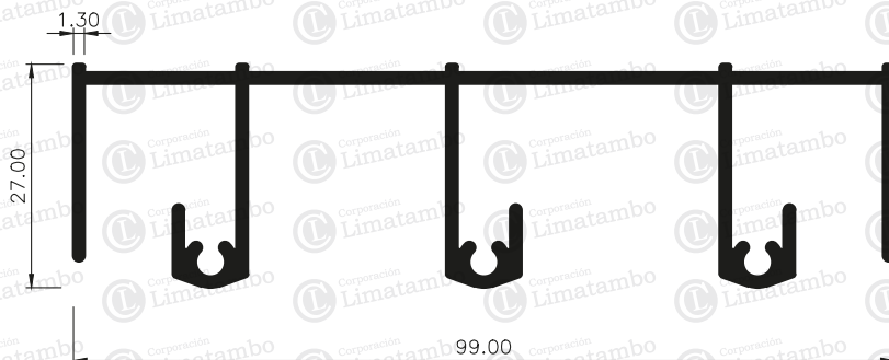
MARCO SUPERIOR TRIPLE CARRIL
