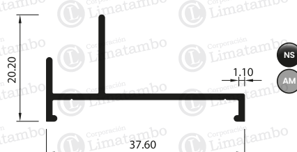
MARCO SUP. FIJA CORREDIZA
