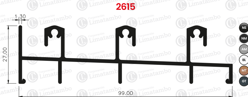
MARCO INFERIOR TRIPLE CARRIL
