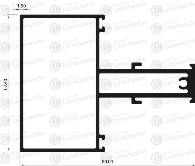
MARCO CENTRAL
