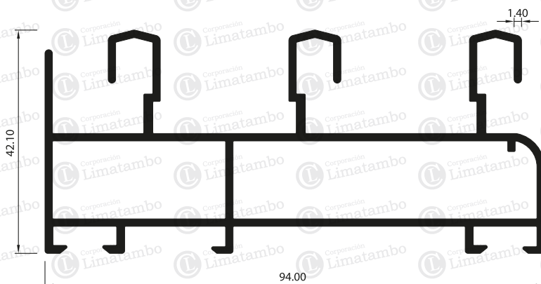
MARCO TRIPLE CORREDIZA
