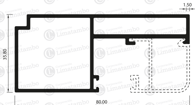
MARCO LATERAL
