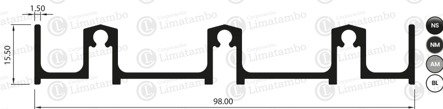
MARCO INFERIOR TRIPLE CARRIL
