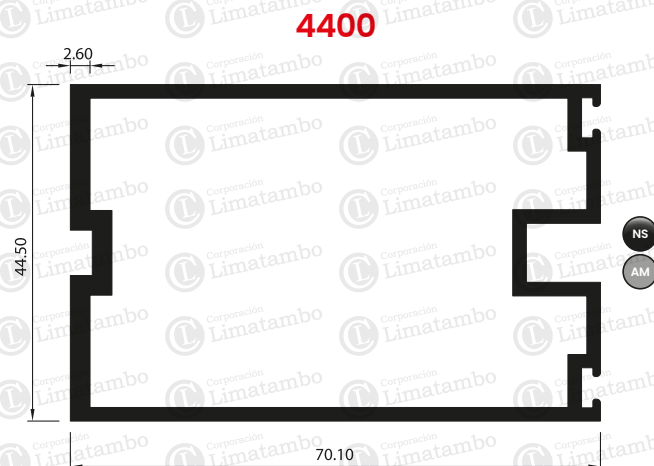
MULLION LIVIANO
