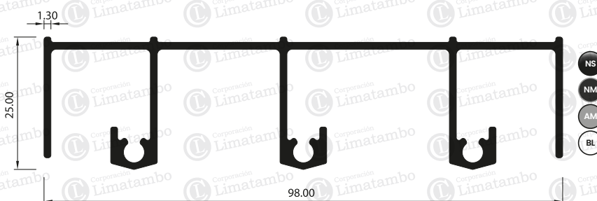
MARCO SUPERIOR TRIPLE CARRIL
