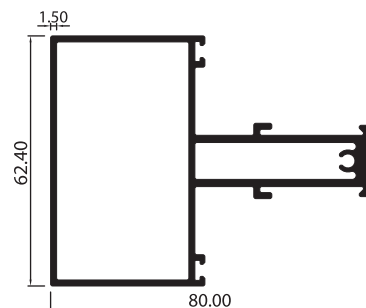
MARCO CENTRAL MBL4602
