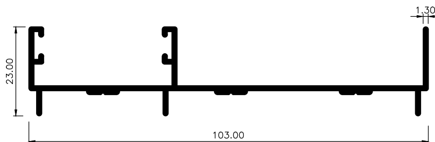
MARCO LATERAL TRIPLE CARRIL 2616
