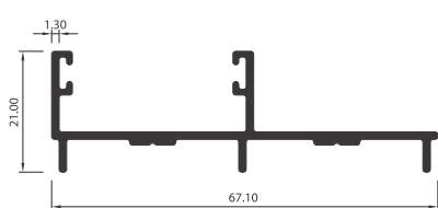
MARCO LATERAL VL4215
