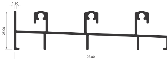
MARCO INFERIOR TRIPLE CARRIL VL4216
