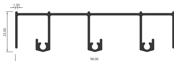
MARCO SUPERIOR TRIPLE CARRIL VL4217
