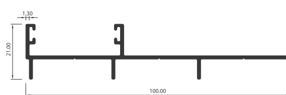
MARCO LATERAL TRIPLE CARRIL VL4218
