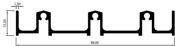
MARCO INFERIOR TRIPLE CARRIL ML4207
