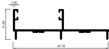
MARCO LATERAL VL4215
