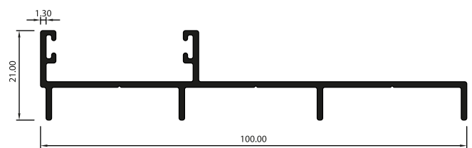
MARCO LATERAL TRIPLE CARRIL VL4218
