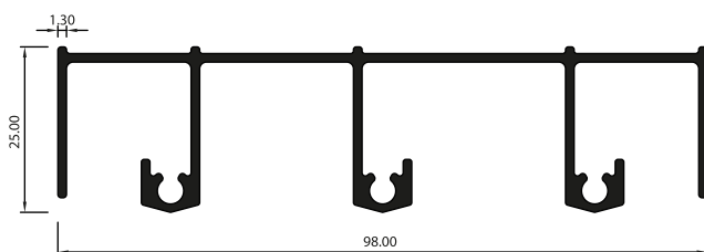
MARCO SUPERIOR TRIPLE CARRIL VL4217
