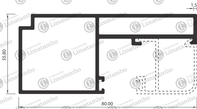
MARCO LATERAL
