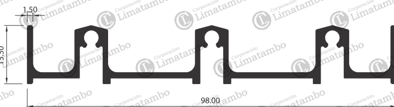
MARCO INFERIOR TRIPLE CARRIL
