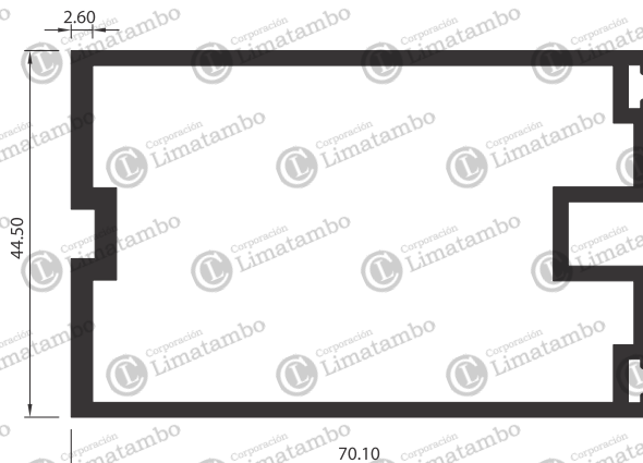
MULLION LIVIANO
