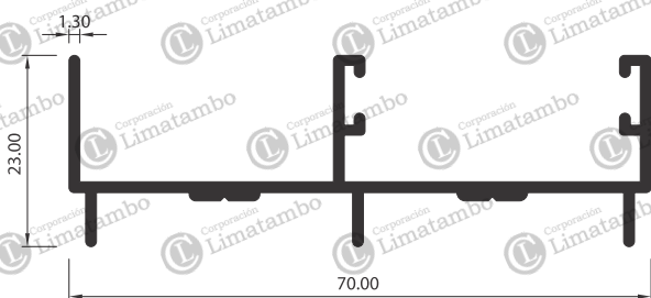
MARCO LATERAL
