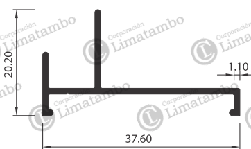
MARCO SUP. FIJA CORREDIZA
