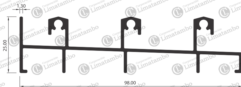
MARCO INFERIOR TRIPLE CARRIL
