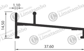
MARCO INF. FIJA CORREDIZA
