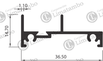
MARCO LATERAL
