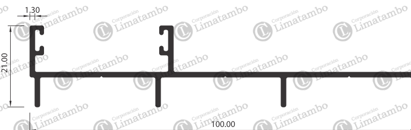
MARCO LATERAL TRIPLE CARRIL
