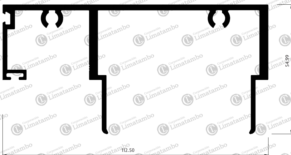
MONTANTE VERTICAL A
