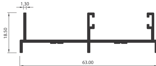
MARCO LATERAL 1909
