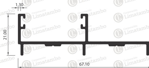
MARCO LATERAL
