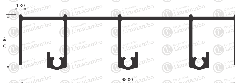
MARCO SUPERIOR TRIPLE CARRIL
