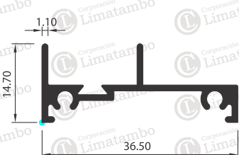
MARCO LATERAL
