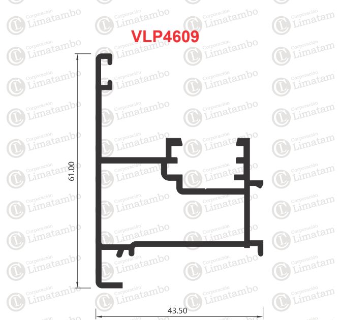
INVERSOR
