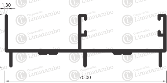
MARCO LATERAL
