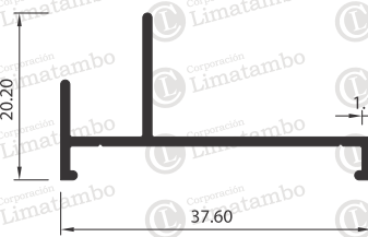
MARCO SUP. FIJA CORREDIZA
