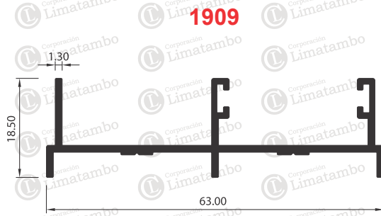
MARCO LATERAL
